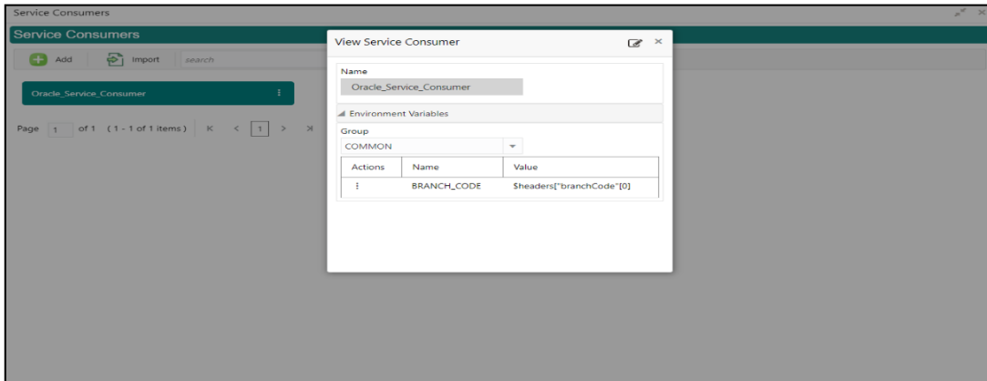
Figure 121: View
