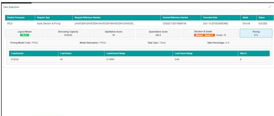
Figure 233 : Pricing Widget
