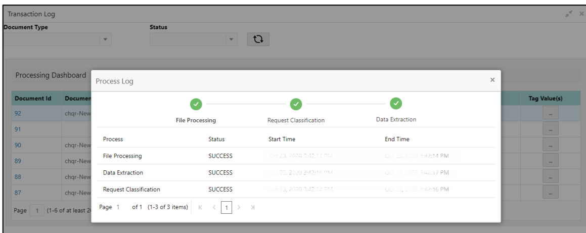
Figure 247: Execution Flow
