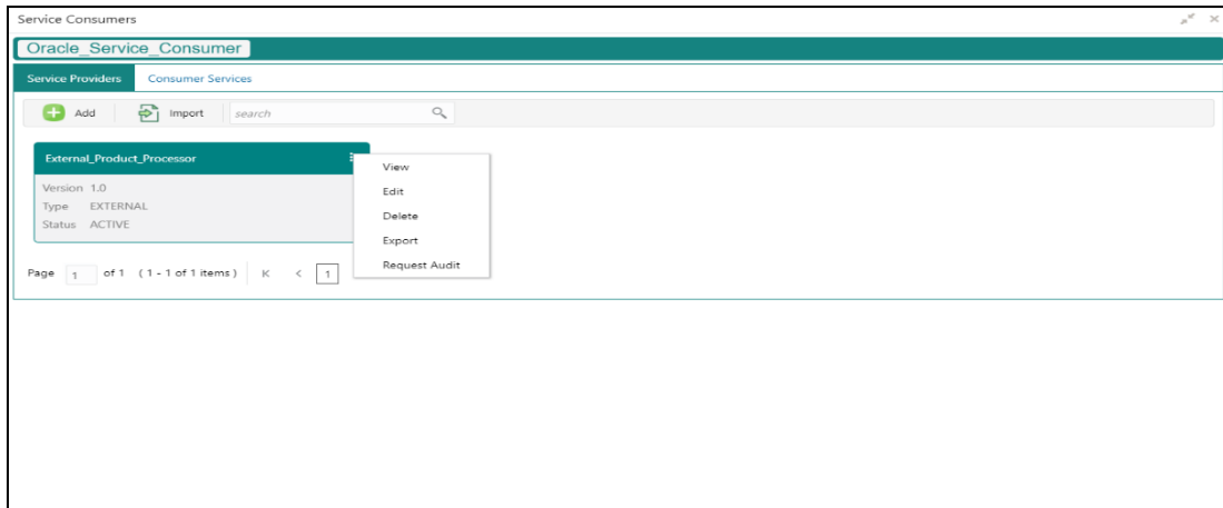
Figure 127: Service Providers
