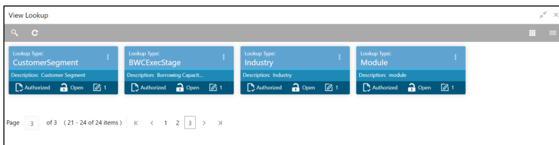
Figure 100 : View Lookup
