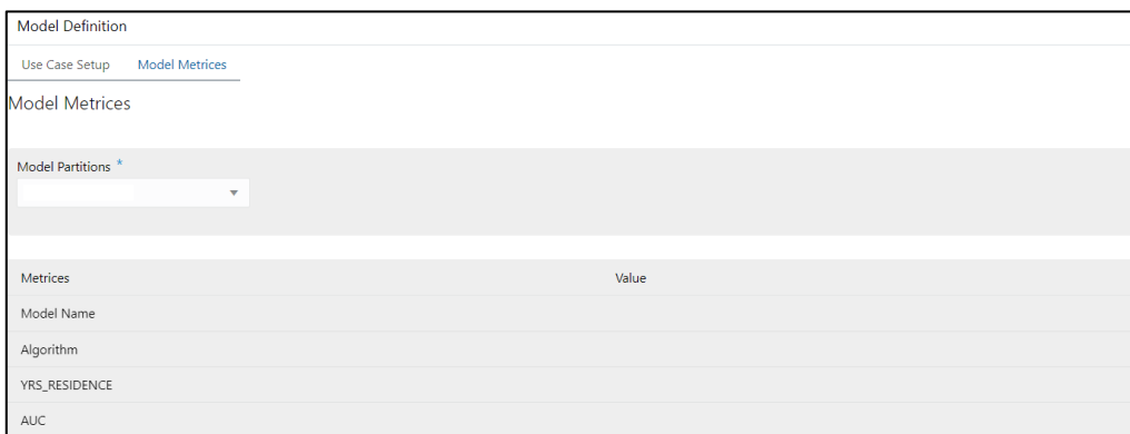
Figure 257: Model Metrics
