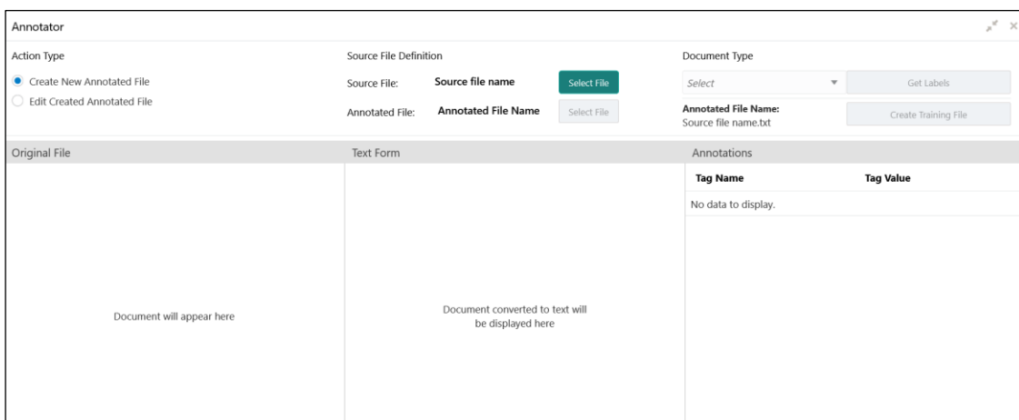
Figure 237: Annotator
